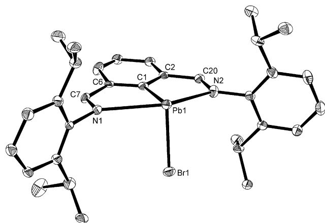
Figure 1. Molecular structure of compound 2 (ellipsoids set at 50% probability). Hydrogen atoms and disorder in the i Pr substituents are omitted for clarity. Selected bond lengths [Å] and angles [°]: Pb1–C1 2.289(19), Pb1–Br1 2.701(2), Pb1–N1 2.637(16), Pb1–N2 2.691(17), N1–C7 1.27(2), N2–C20 1.25(3), C2–C20 1.46(3), C6–C7 1.48(3), C1–C6 1.36(3), C1–C2 1.38(3); C1–Pb1–Br1 95.0(4), C1–Pb1–N1 68.6(6), C1–Pb1–N2 68.0(6), N1–Pb1–N2 135.9(5), N1–Pb1–Br1 88.1(4), N2–Pb1–Br1 88.2(4).
